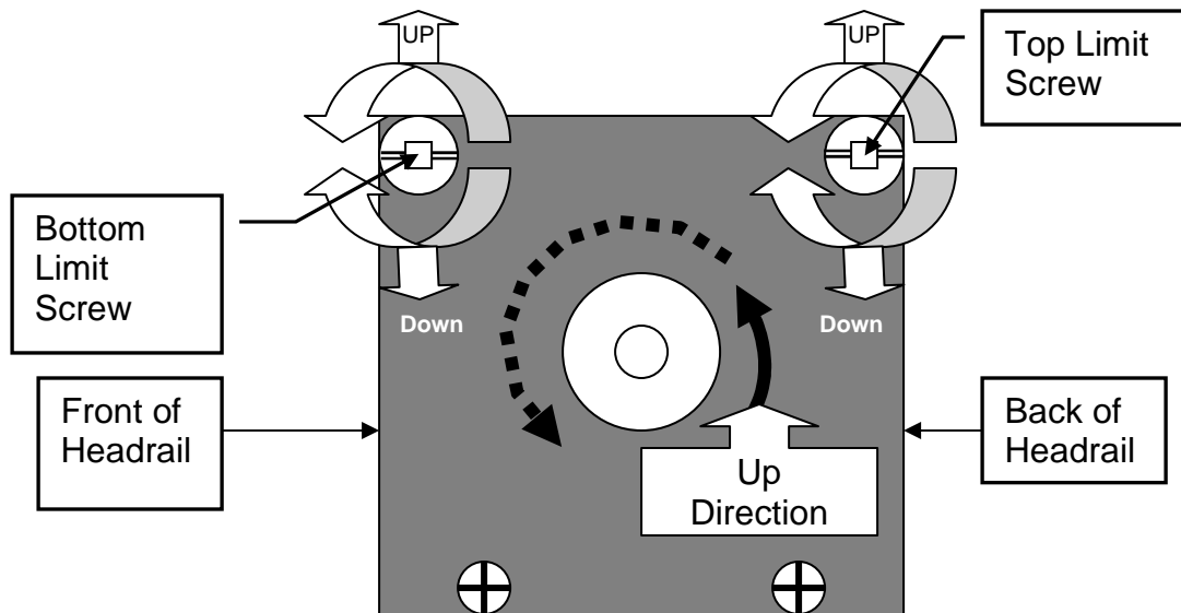
Fig.1 Limit switch is shown on right side of headrail
